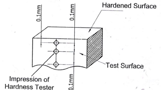
Transverse For Hardness Check
